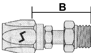
INVERTED FLARE SWIVEL
