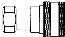
PHH862 Female Thread Coupler - Steel Body Size: 1"; Thread Size NPTF: 1-11-1/2; For Use with PHH863; 1 per package
