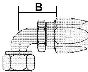
90° ELBOW SWIVEL SAE 37°/45° PTT 30° FLARE
