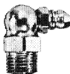
CN613 1/8" Pipe Thread; 13/16" Length; 90° Elbow; Ball Check
