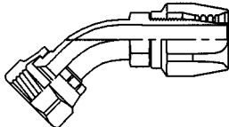
PH2372188 Female JIC 37° - Swivel; 45° Elbow - Short Drop; 1/2" Thread;
